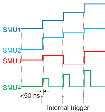
Figure 12. Internal trigger lines enable channel synchronization at less than 50 ns accuracy, and external trigger ports enable synchronization with any piece of external equipment
