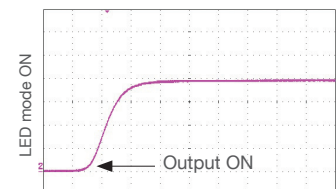
Current flow during power up with LED mode enabled
